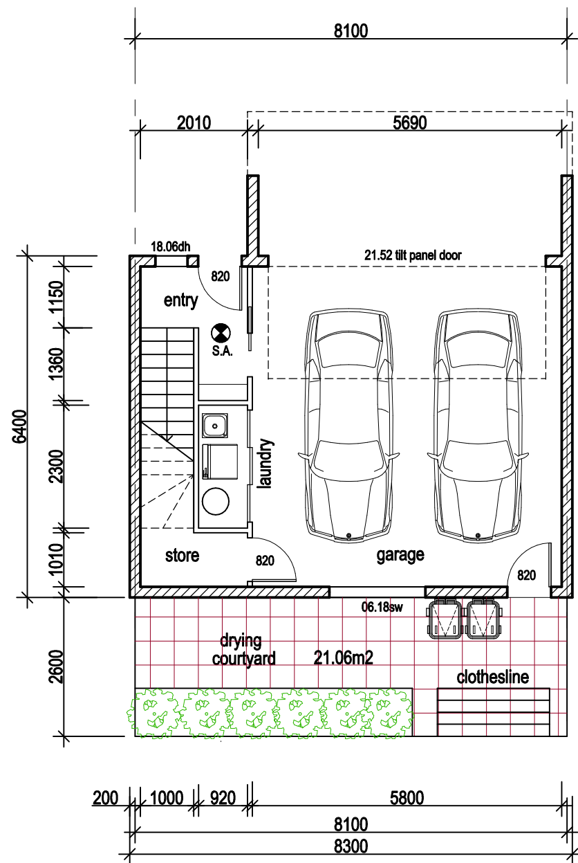
GROUND FLOOR gfa = 8.85m 2
