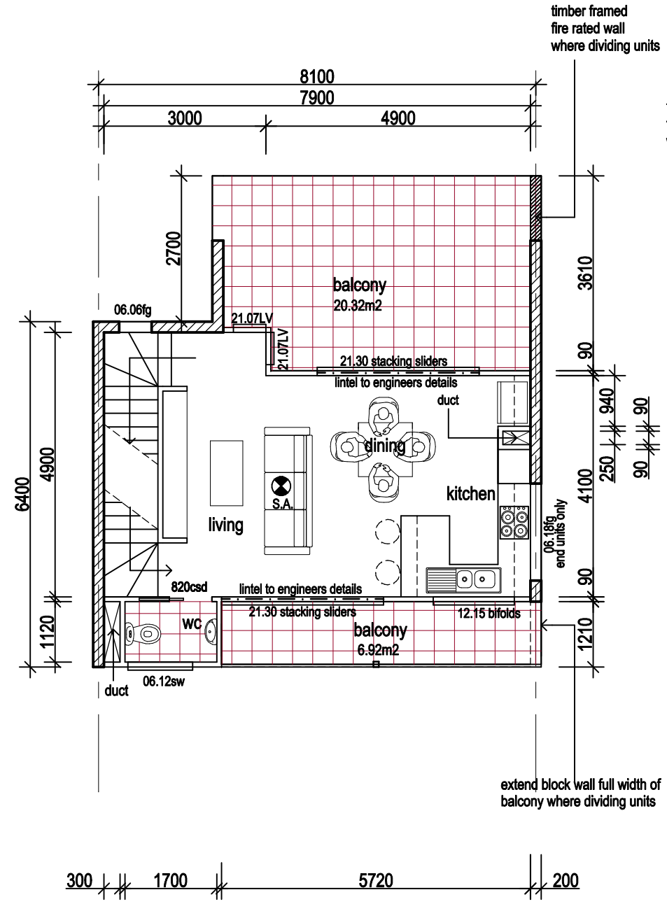
FIRST FLOOR gfa = 34.03m 2
